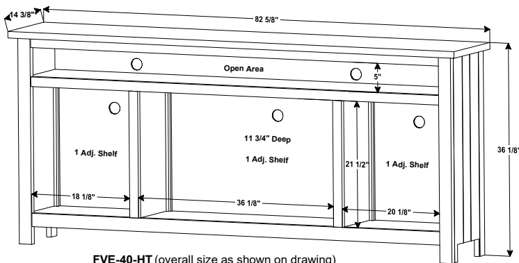
FVE-40-HT (overall size as shown on drawing) FVE-40-A (overall size = 85 1/4"W x 14 7/8"D x 39 1/4"H) FVE-40-BC (overall size = 83 3/8"W x 15"D x 36"H) FVE-40-D (overall size = 82 5/8"W x 14"D x 35 7/8"H) FVE-40-EN (overall size = 85 7/8"W x 14 1/2"D x 38"H) FVE-40-LA (overall size = 84 5/8"W x 15 1/2"D x 36"H)
