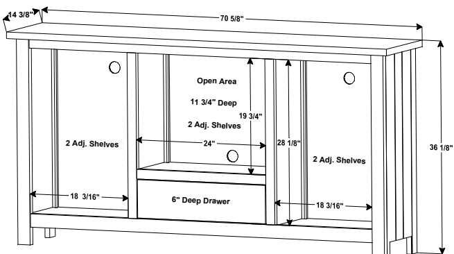
FVE-26-HT (overall size as shown on drawing) FVE-26-A (overall size = 73 1/4"W x 14 7/8"D x 39 1/4"H) FVE-26-BC (overall size = 71 3/8"W x 15"D x 36"H) FVE-26-D (overall size = 70 5/8"W x 14"D x 35 7/8"H) FVE-26-EN (overall size = 73 7/8"W x 14 1/2"D x 38"H) FVE-26-LA (overall size = 72 5/8"W x 15 1/2"D x 36"H)
