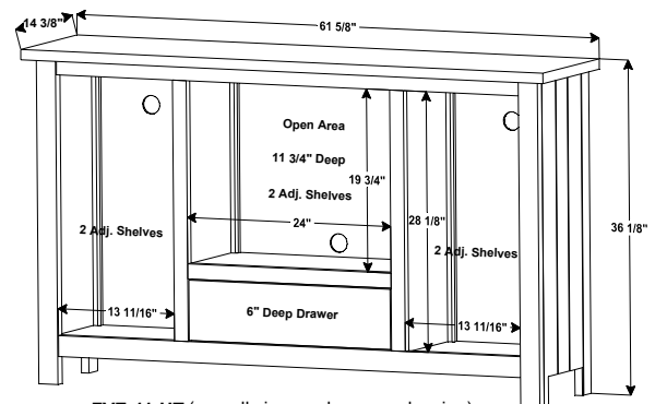
FVE-11-HT (overall size as shown on drawing) FVE-11-A (overall size = 64 1/4"W x 14 7/8"D x 39 1/4"H) FVE-11-BC (overall size = 62 3/8"W x 15"D x 36"H) FVE-11-D (overall size = 61 5/8"W x 14"D x 35 7/8"H) FVE-11-EN (overall size = 64 7/8"W x 14 1/2"D x 38"H) FVE-11-LA (overall size = 63 5/8"W x 15 1/2"D x 36"H)
