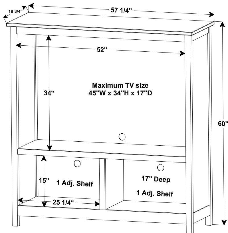
FVE-05-CN TV sits 21 1/4" off the floor
