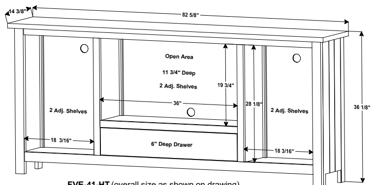
FVE-41-HT (overall size as shown on drawing) FVE-41-A (overall size = 85 1/4"W x 14 7/8"D x 39 1/4"H) FVE-41-BC (overall size = 83 3/8"W x 15"D x 36"H) FVE-41-D (overall size = 82 5/8"W x 14"D x 35 7/8"H) FVE-41-EN (overall size = 85 7/8"W x 14 1/2"D x 38"H) FVE-41-LA (overall size = 84 5/8"W x 15 1/2"D x 36"H)
