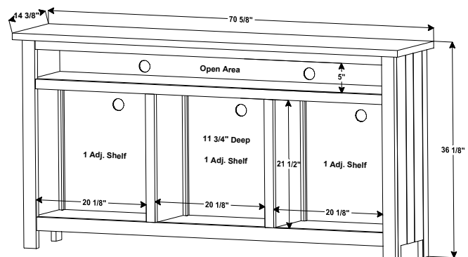
FVE-25-HT (overall size as shown on drawing) FVE-25-A (overall size = 73 1/4"W x 14 7/8"D x 39 1/4"H) FVE-25-BC (overall size = 71 3/8"W x 15"D x 36"H) FVE-25-D (overall size = 70 5/8"W x 14"D x 35 7/8"H) FVE-25-EN (overall size = 73 7/8"W x 14 1/2"D x 38"H) FVE-25-LA (overall size = 72 5/8"W x 15 1/2"D x 36"H)
