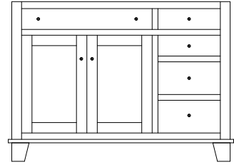
IS-2074 47¼"w 34½"h 24"d w/5 drawers 2 doors w/1 adjustable shelf
